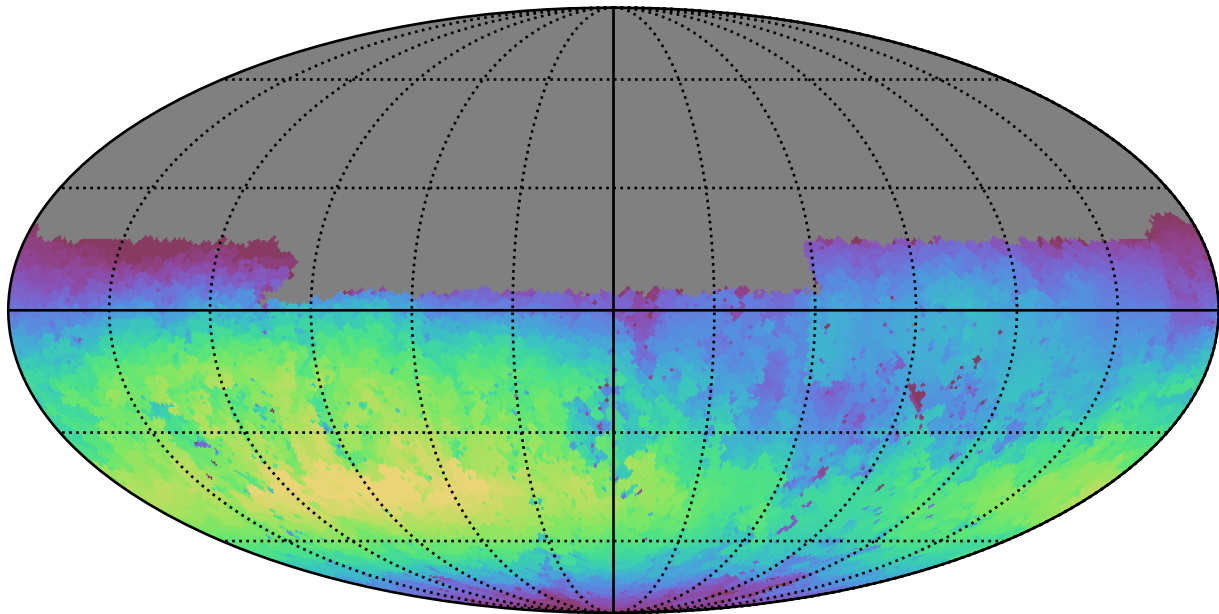
no_high_blob_v3.3_10yrs Yr 1 u band: Max skyBrightness
