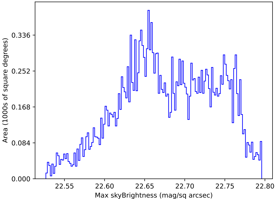
no_high_blob_v3.3_10yrs Yr 1 u band: Max skyBrightness
