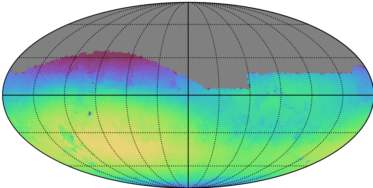
no_high_blob_v3.3_10yrs Yr 1 r band: Max skyBrightness
