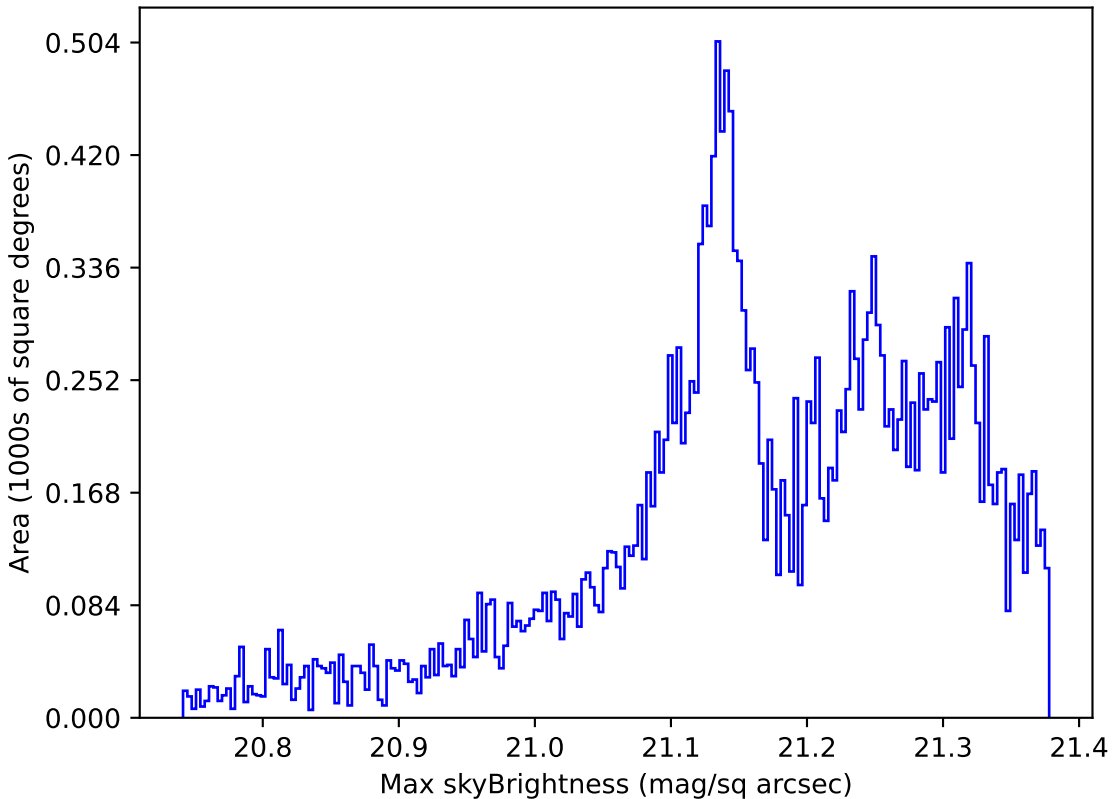
no_high_blob_v3.3_10yrs Yr 1 r band: Max skyBrightness
