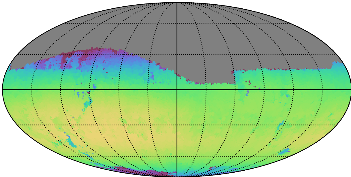
no_high_blob_v3.3_10yrs Yr 1 i band: Max skyBrightness
