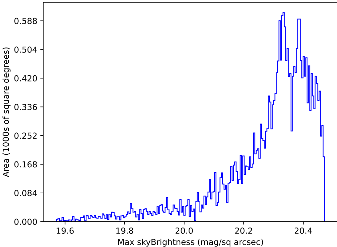
no_high_blob_v3.3_10yrs Yr 1 i band: Max skyBrightness
