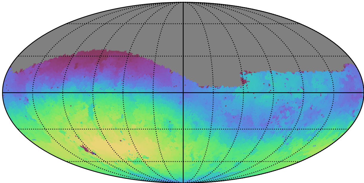
no_high_blob_v3.3_10yrs Yr 1 g band: Max skyBrightness
