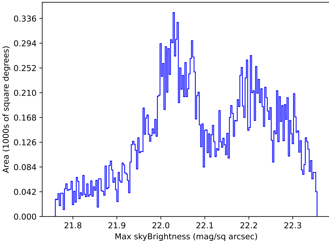
no_high_blob_v3.3_10yrs Yr 1 g band: Max skyBrightness
