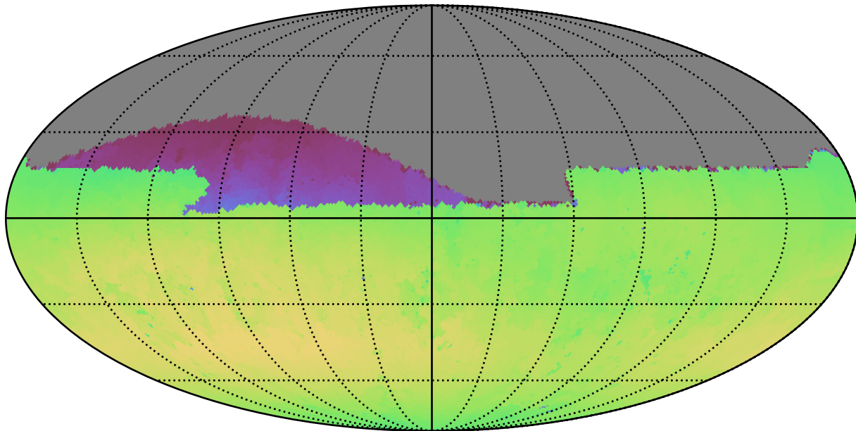
no_high_blob_v3.3_10yrs Yr 1 all bands: Max skyBrightness
