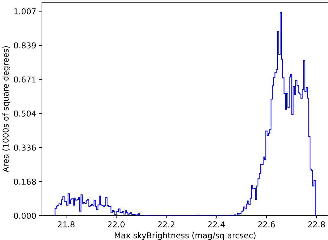
no_high_blob_v3.3_10yrs Yr 1 all bands: Max skyBrightness
