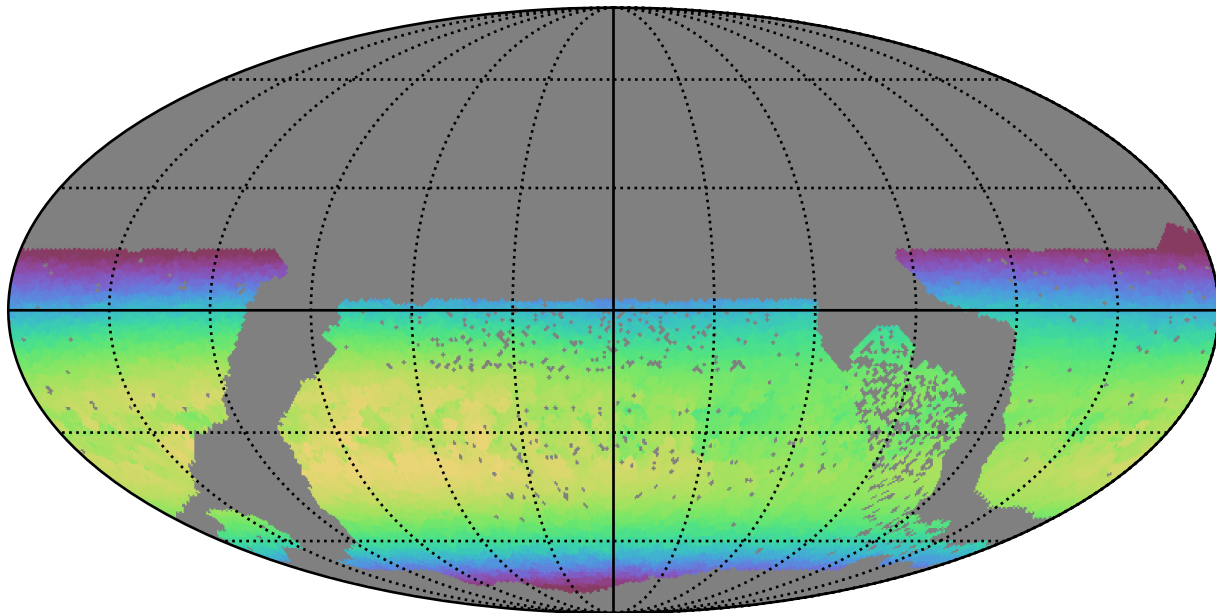
no_high_blob_v3.3_10yrs WFD z band: Max skyBrightness
