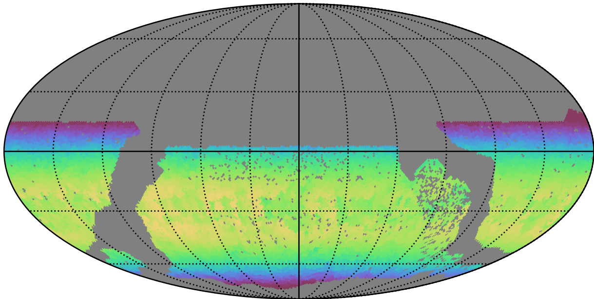
no_high_blob_v3.3_10yrs WFD y band: Max skyBrightness
