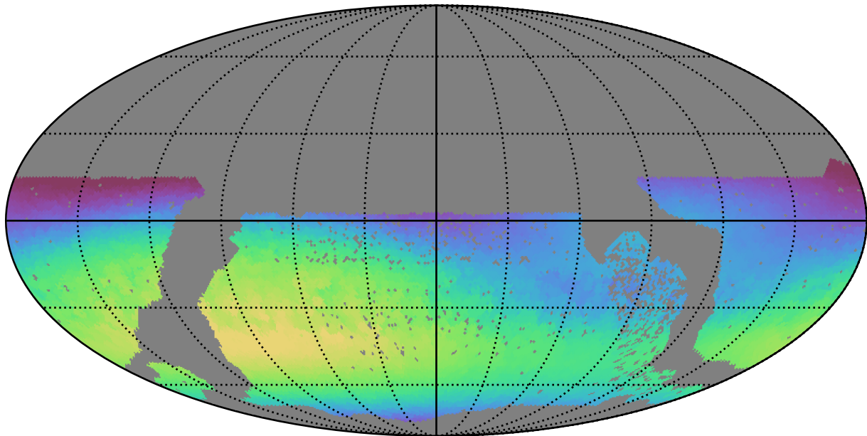
no_high_blob_v3.3_10yrs WFD u band: Max skyBrightness
