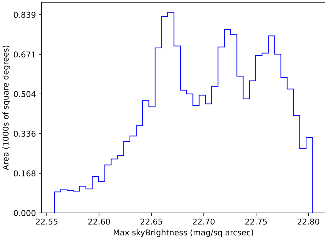
no_high_blob_v3.3_10yrs WFD u band: Max skyBrightness
