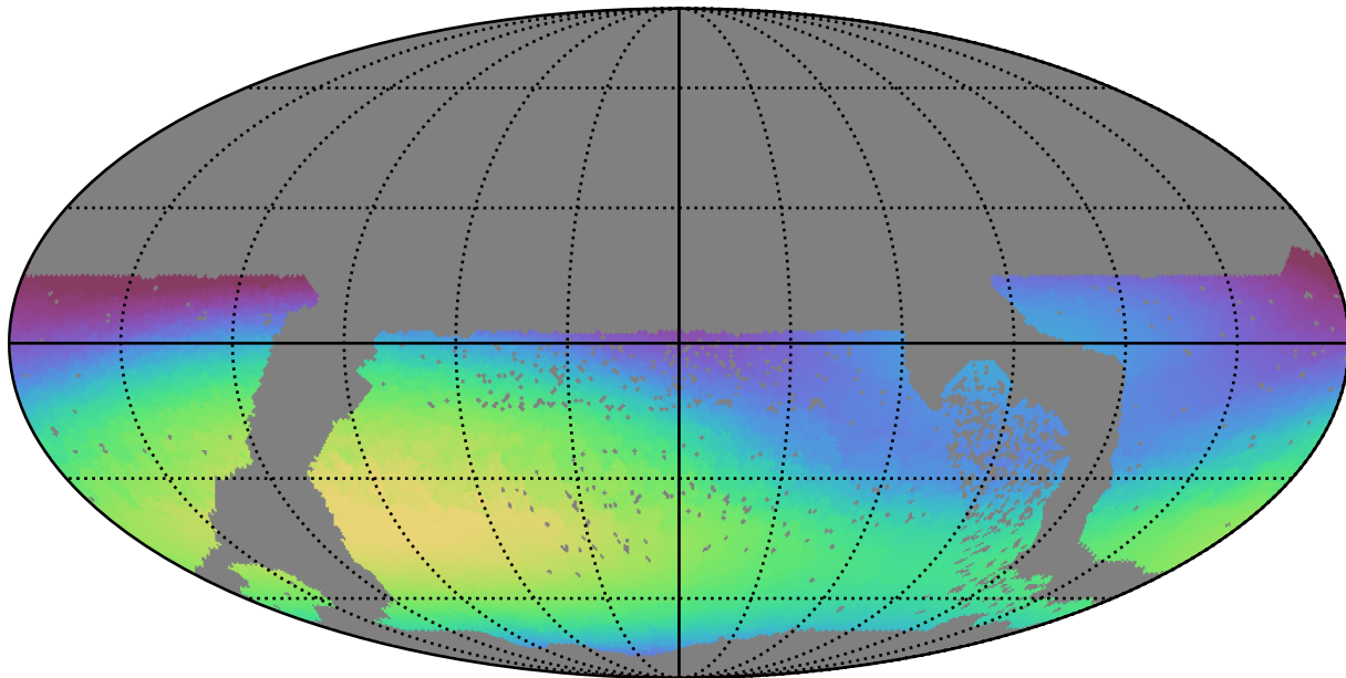
no_high_blob_v3.3_10yrs WFD r band: Max skyBrightness
