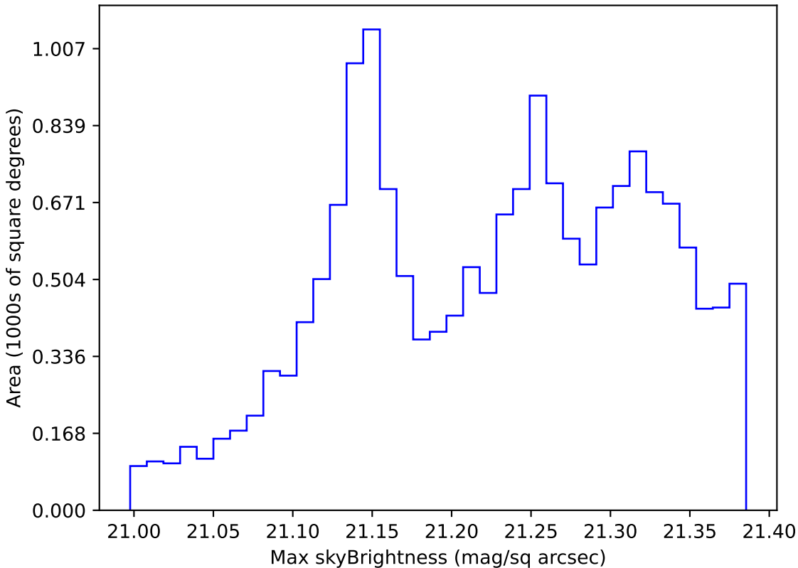
no_high_blob_v3.3_10yrs WFD r band: Max skyBrightness
