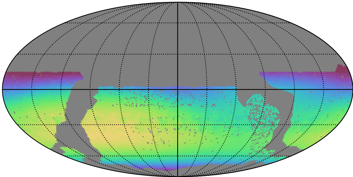
no_high_blob_v3.3_10yrs WFD i band: Max skyBrightness
