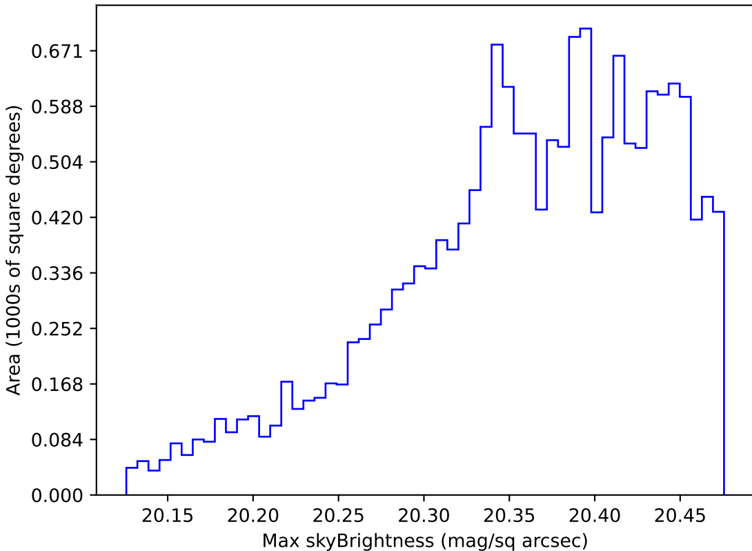
no_high_blob_v3.3_10yrs WFD i band: Max skyBrightness
