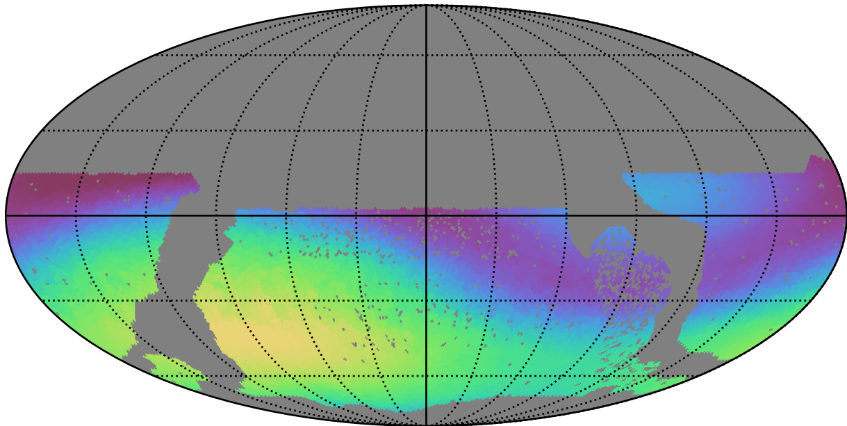
no_high_blob_v3.3_10yrs WFD g band: Max skyBrightness
