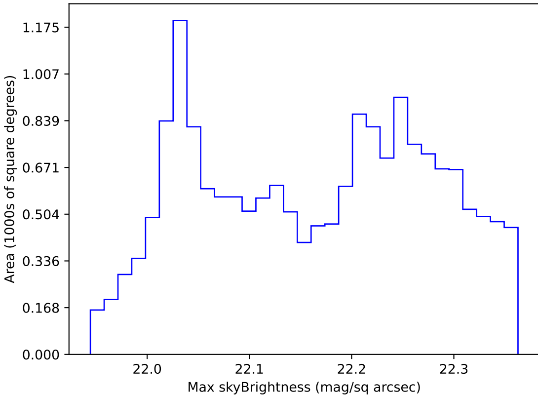
no_high_blob_v3.3_10yrs WFD g band: Max skyBrightness
