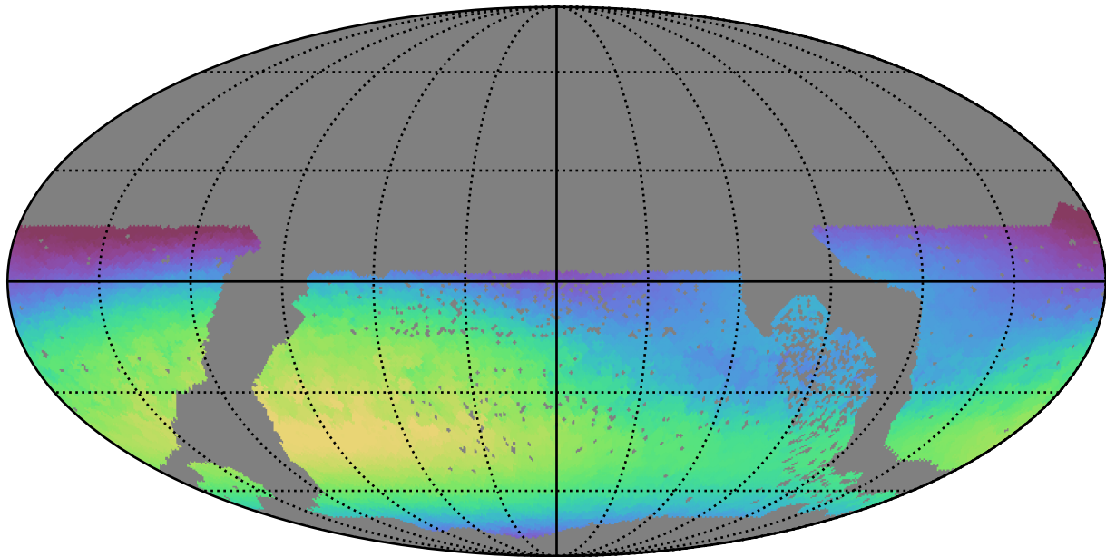
no_high_blob_v3.3_10yrs WFD all bands: Max skyBrightness
