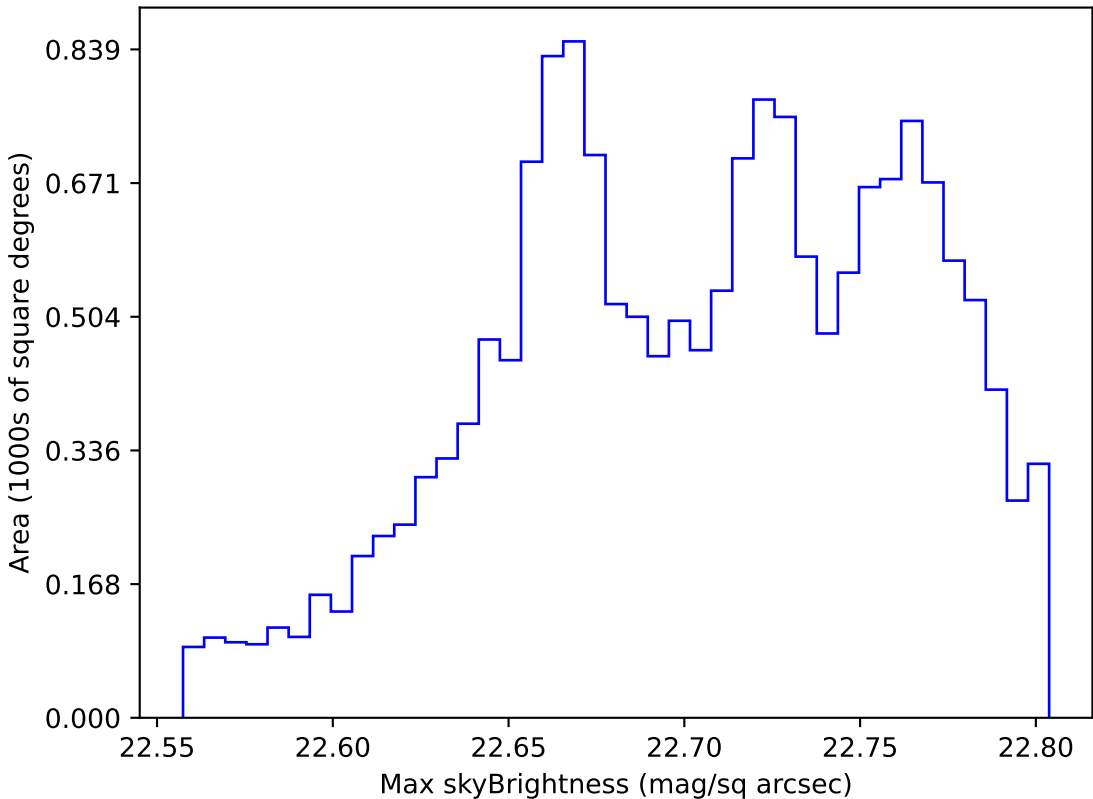
no_high_blob_v3.3_10yrs WFD all bands: Max skyBrightness
