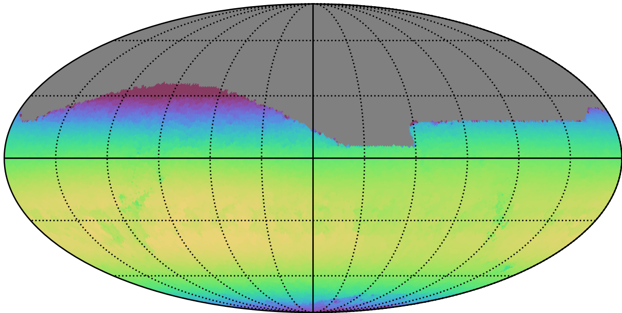
no_high_blob_v3.3_10yrs All sky z band: Max skyBrightness
