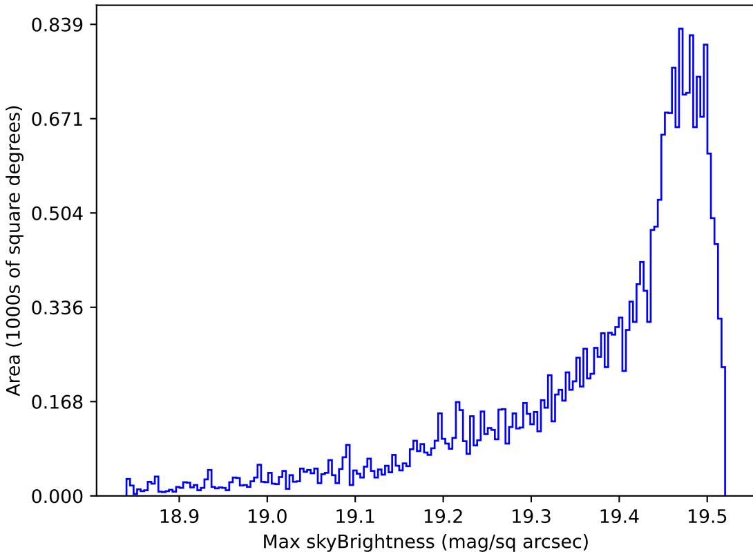
no_high_blob_v3.3_10yrs All sky z band: Max skyBrightness
