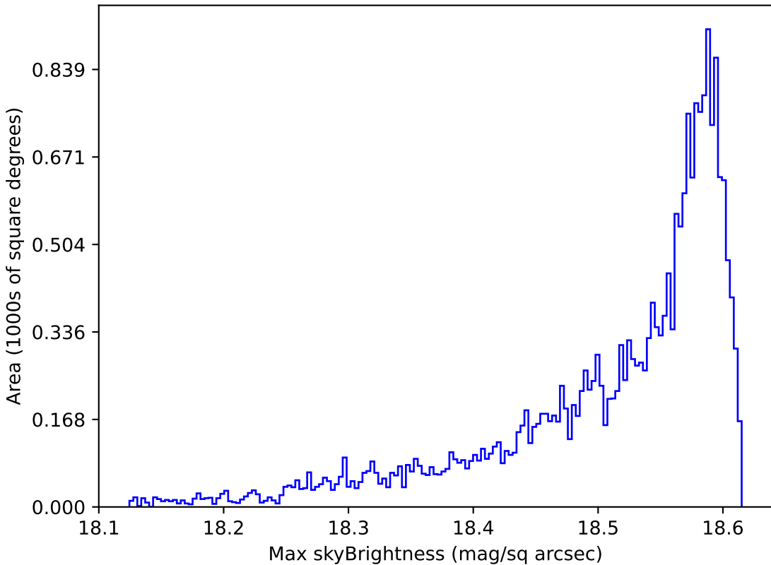
no_high_blob_v3.3_10yrs All sky y band: Max skyBrightness
