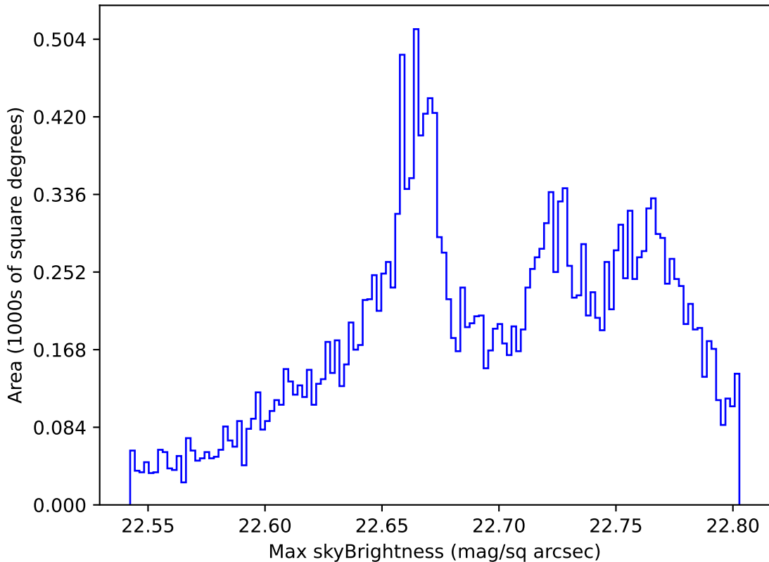
no_high_blob_v3.3_10yrs All sky u band: Max skyBrightness
