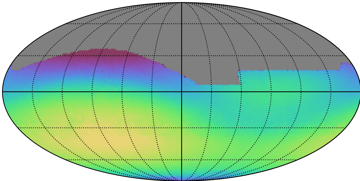
no_high_blob_v3.3_10yrs All sky r band: Max skyBrightness
