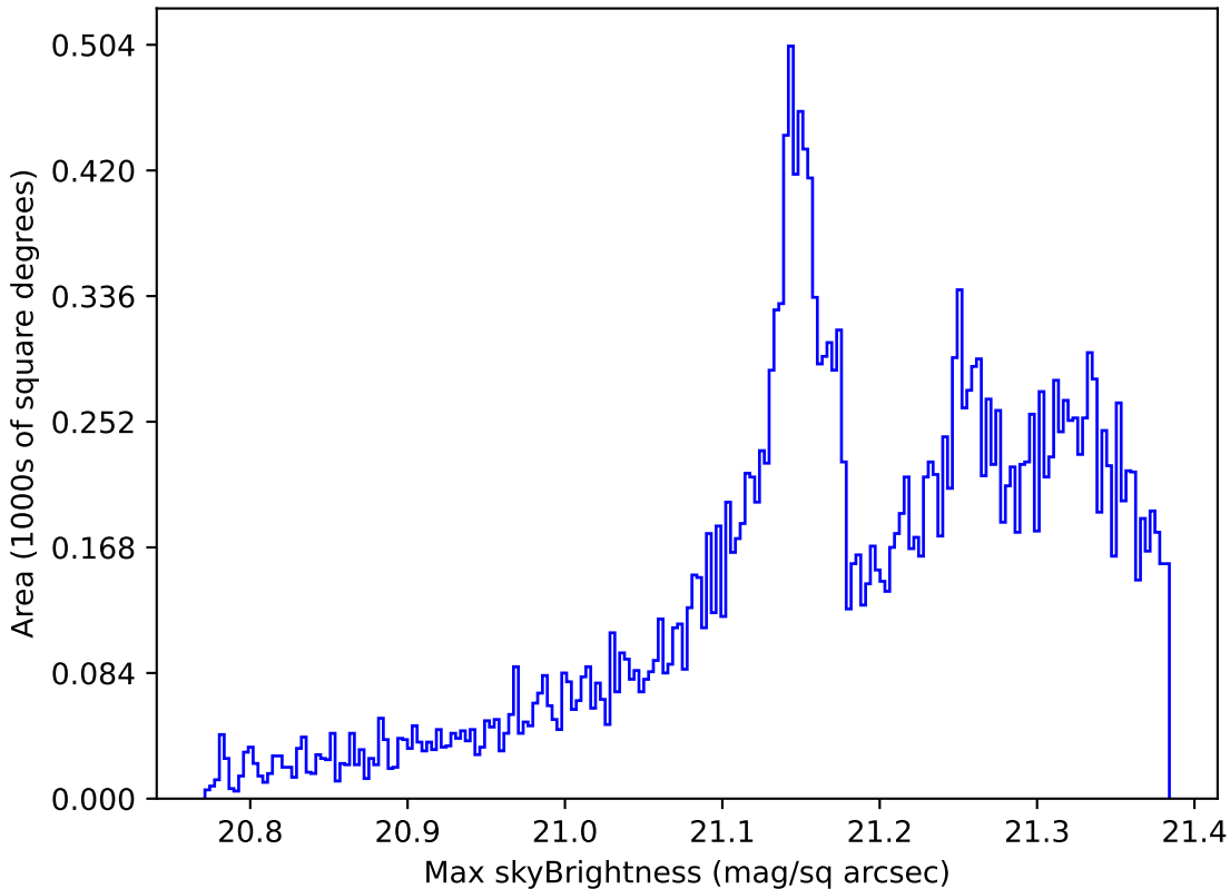
no_high_blob_v3.3_10yrs All sky r band: Max skyBrightness
