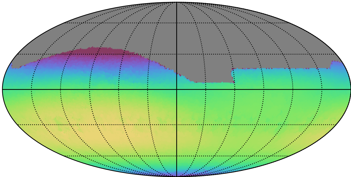
no_high_blob_v3.3_10yrs All sky i band: Max skyBrightness
