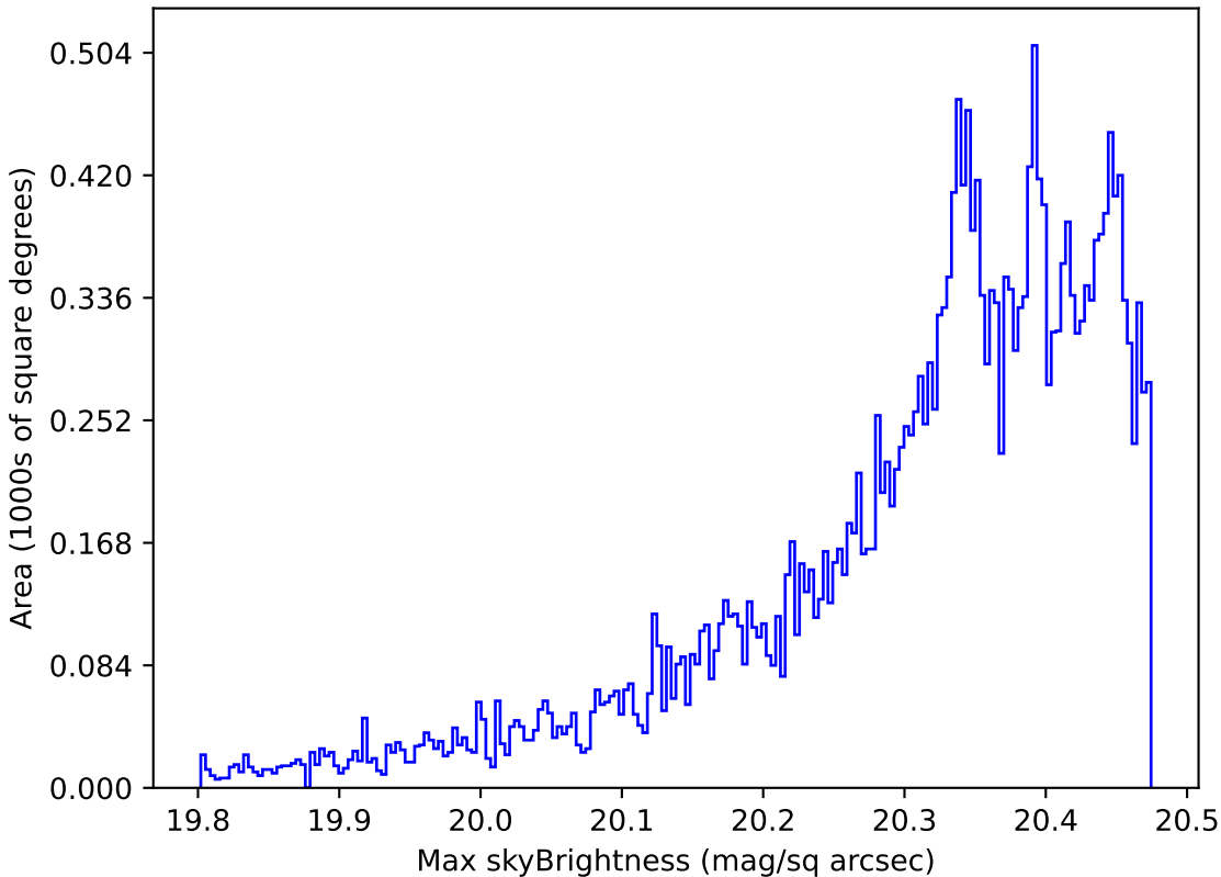
no_high_blob_v3.3_10yrs All sky i band: Max skyBrightness
