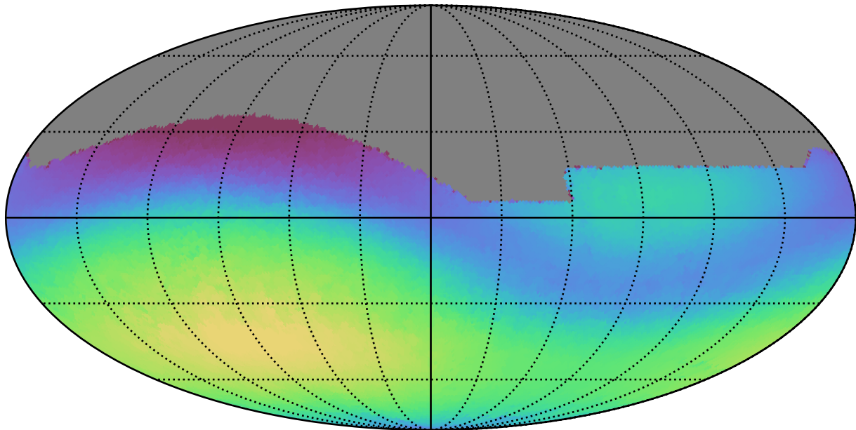
no_high_blob_v3.3_10yrs All sky g band: Max skyBrightness
