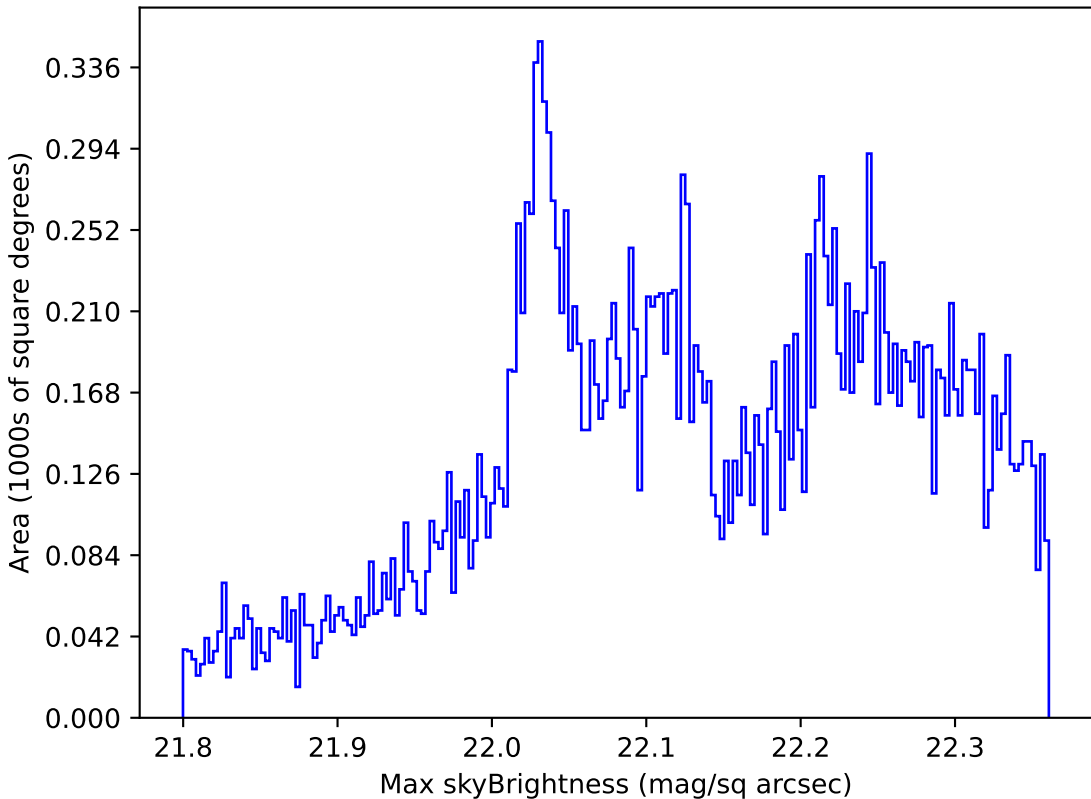
no_high_blob_v3.3_10yrs All sky g band: Max skyBrightness
