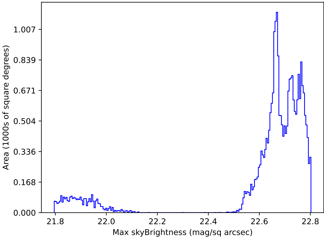
no_high_blob_v3.3_10yrs All sky all bands: Max skyBrightness
