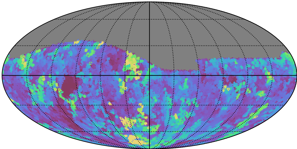
no_high_blob_v3.3_10yrs Yr 1 z band: Max seeingGeom
