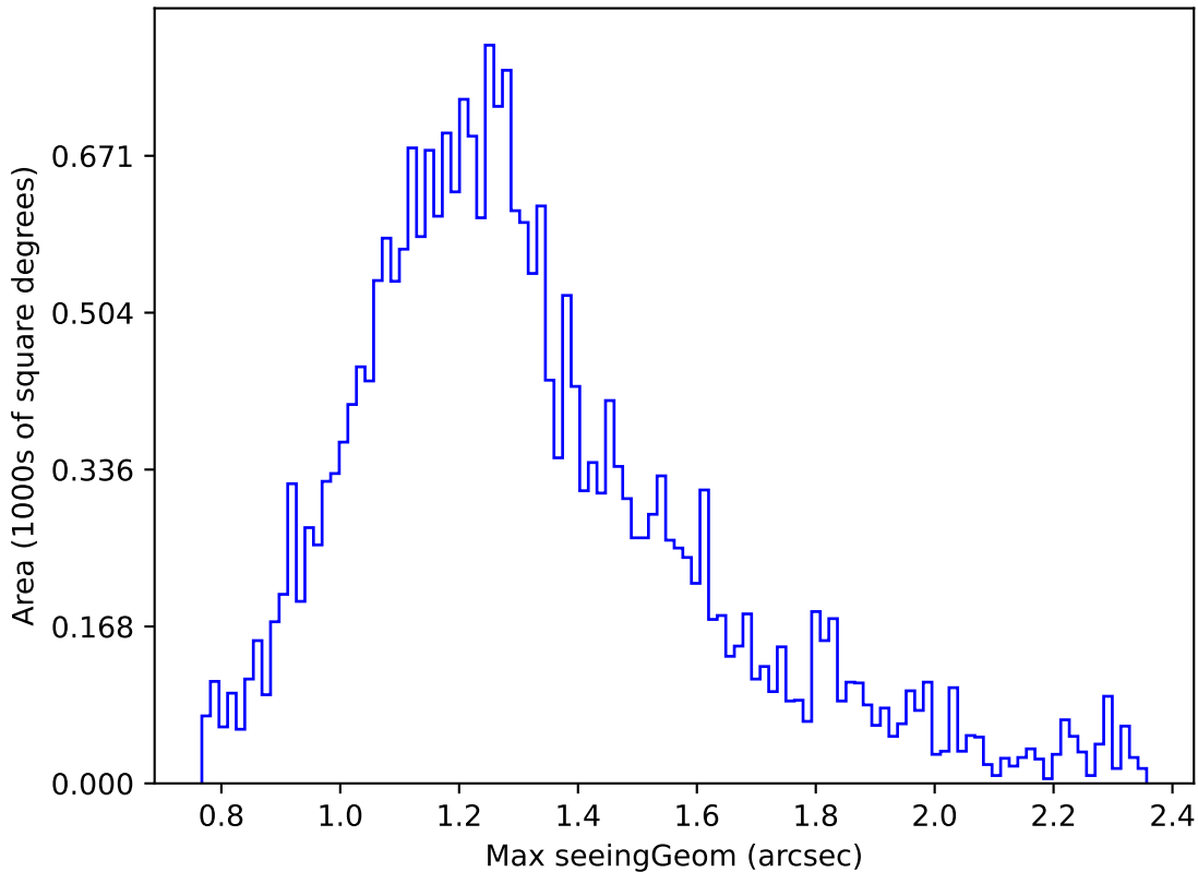
no_high_blob_v3.3_10yrs Yr 1 z band: Max seeingGeom
