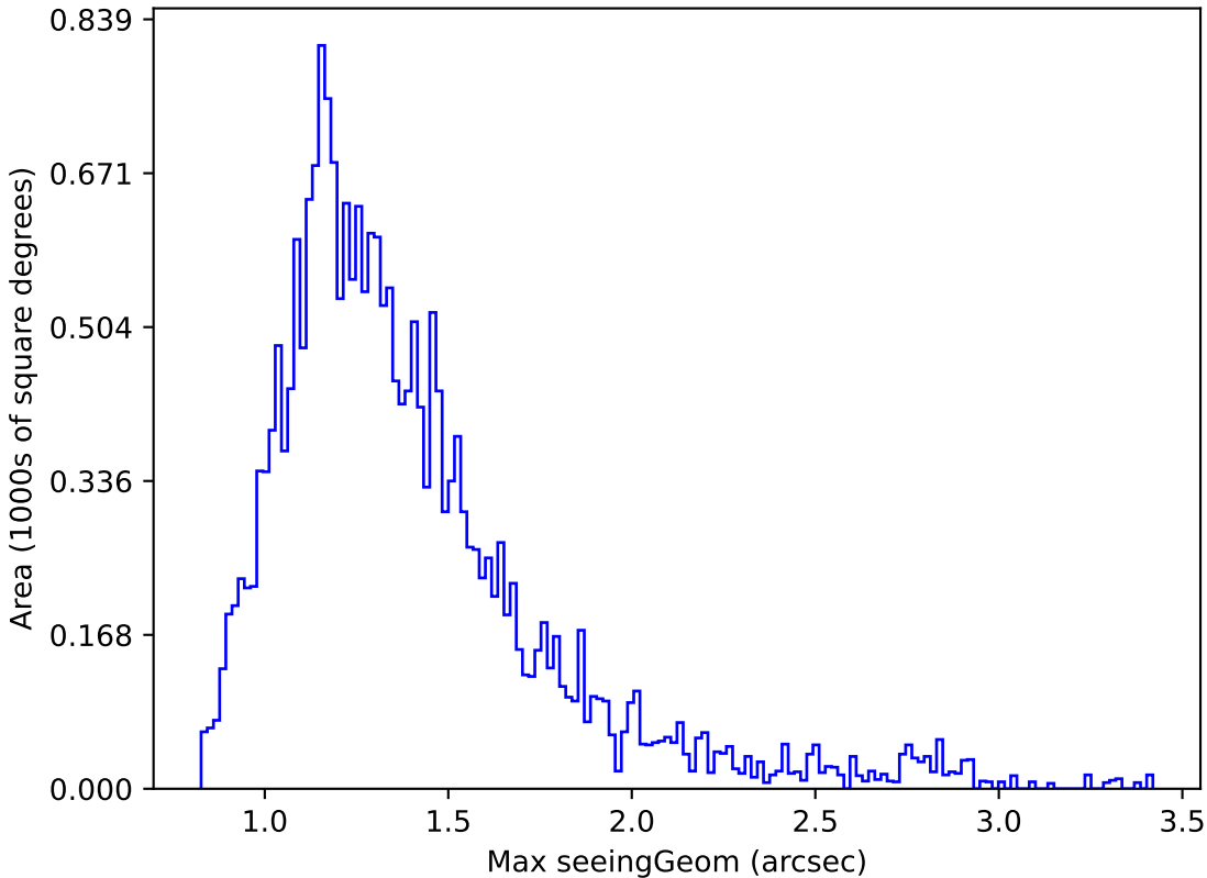
no_high_blob_v3.3_10yrs Yr 1 u band: Max seeingGeom
