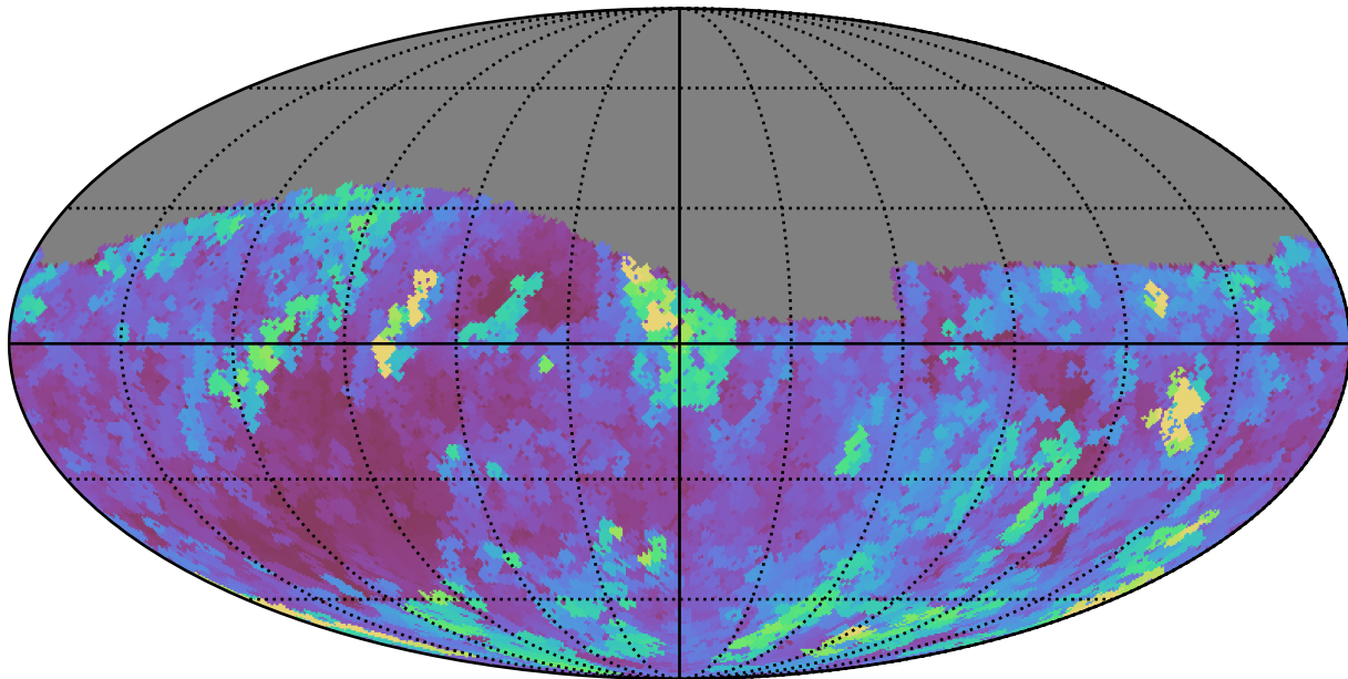
no_high_blob_v3.3_10yrs Yr1 r band: Max seeingGeom
