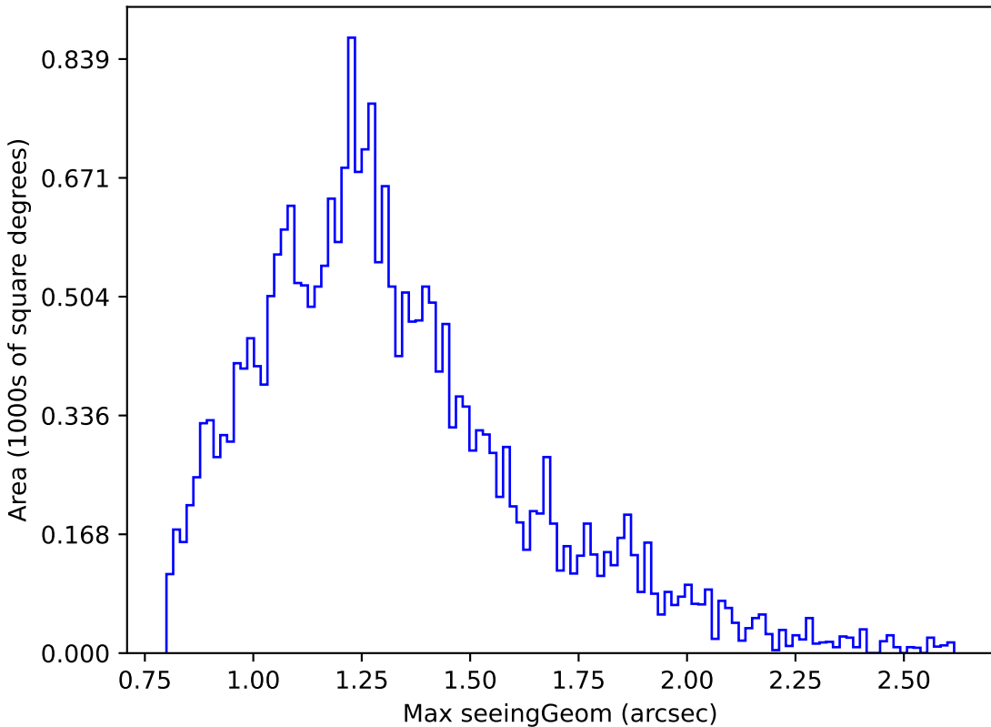
no_high_blob_v3.3_10yrs Yr 1 r band: Max seeingGeom
