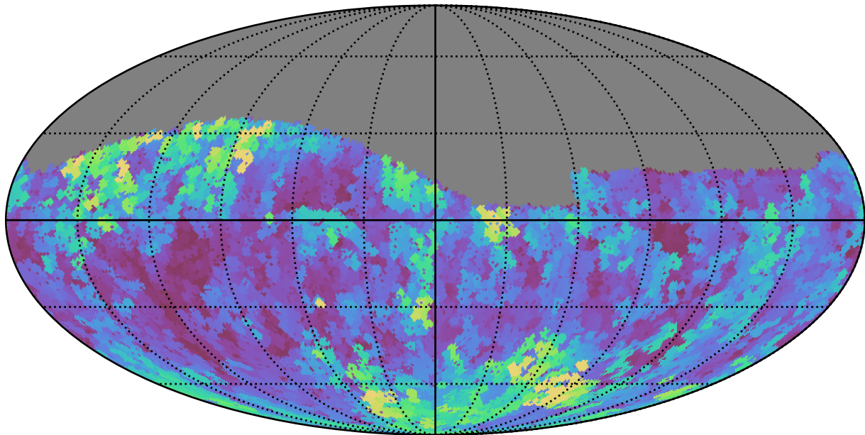
no_high_blob_v3.3_10yrs Yr 1 g band: Max seeingGeom
