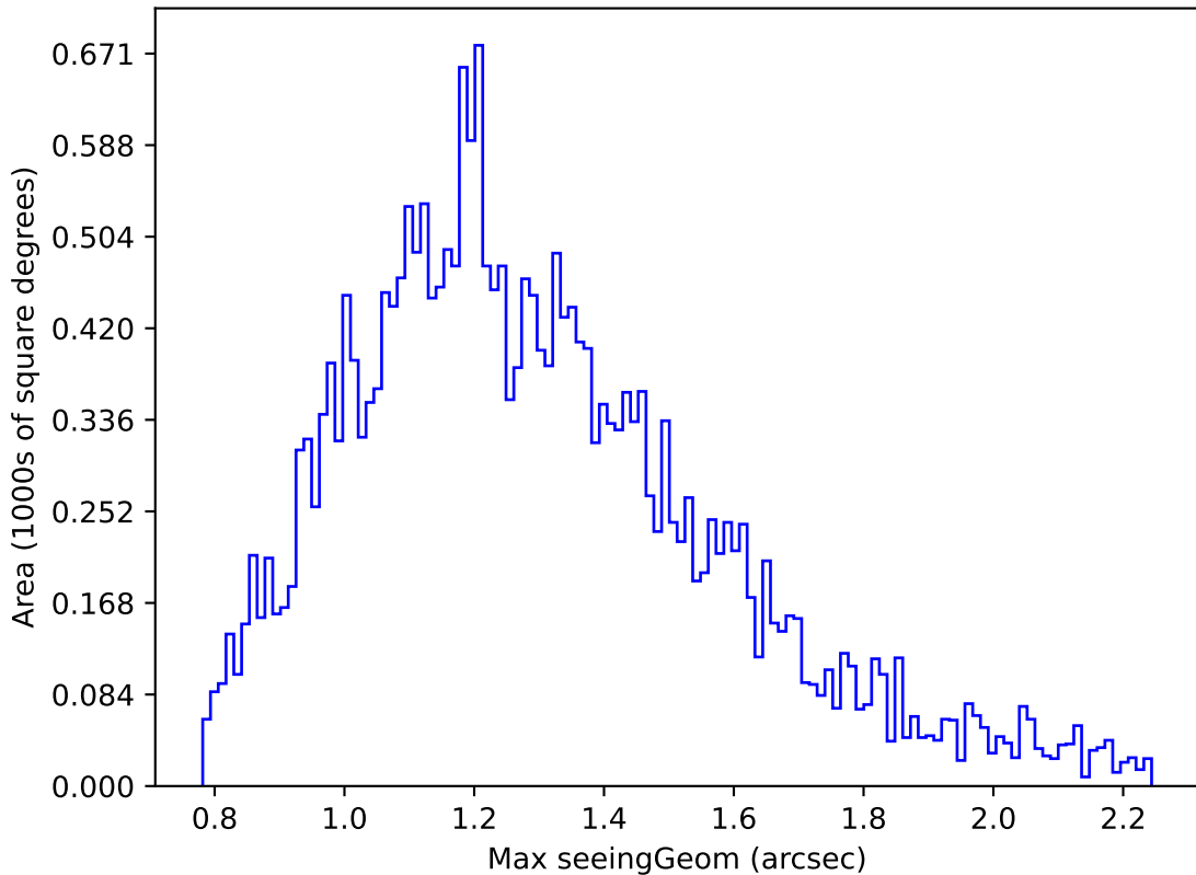
no_high_blob_v3.3_10yrs Yr 1 g band: Max seeingGeom
