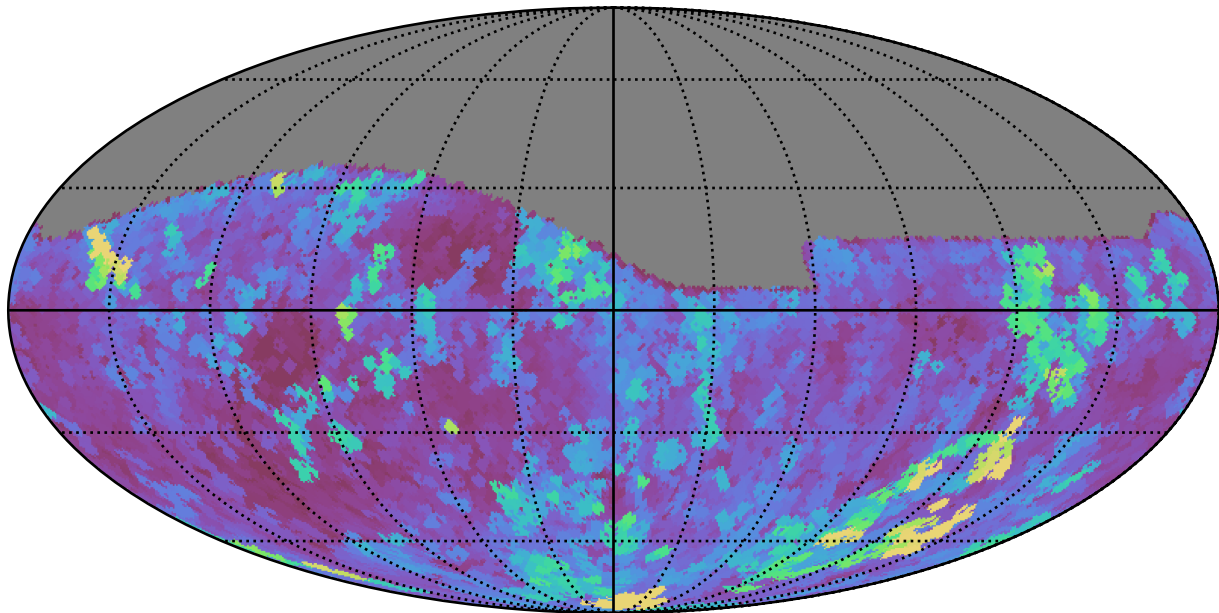
no_high_blob_v3.3_10yrs Yr 1 all bands: Max seeingGeom
