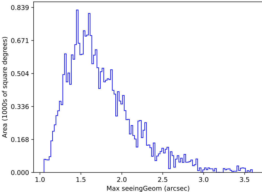
no_high_blob_v3.3_10yrs Yr 1 all bands: Max seeingGeom
