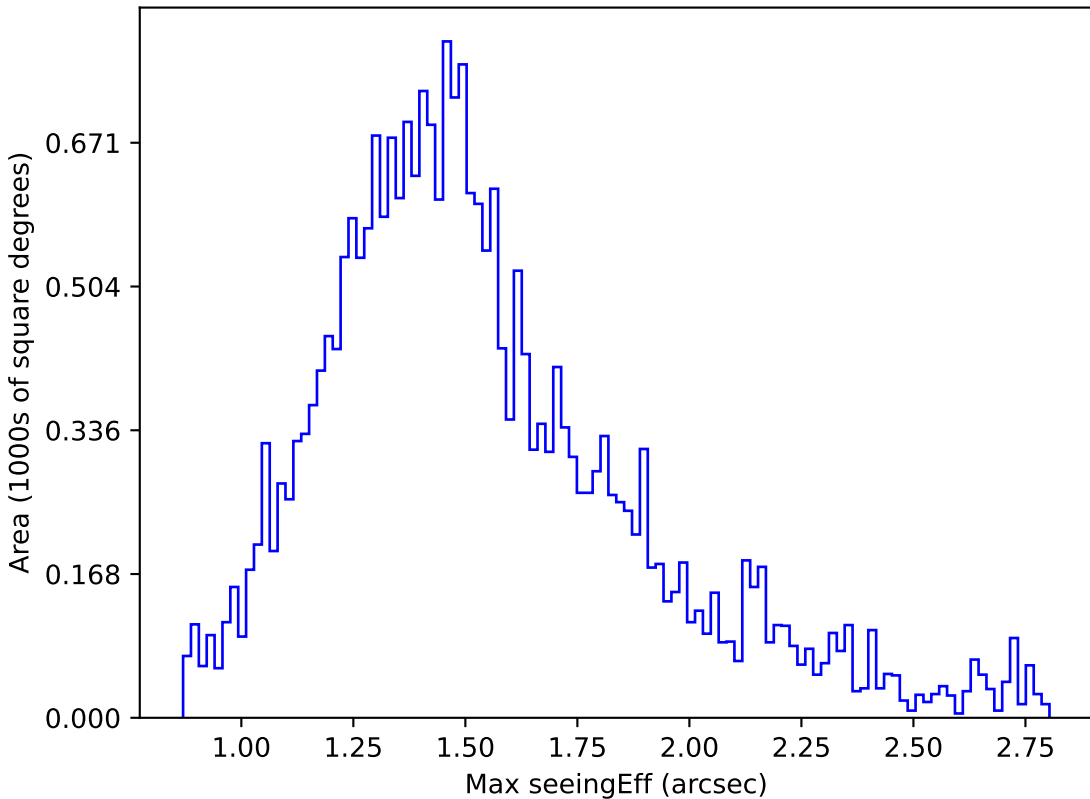
no_high_blob_v3.3_10yrs Yr 1 z band: Max seeingEff
