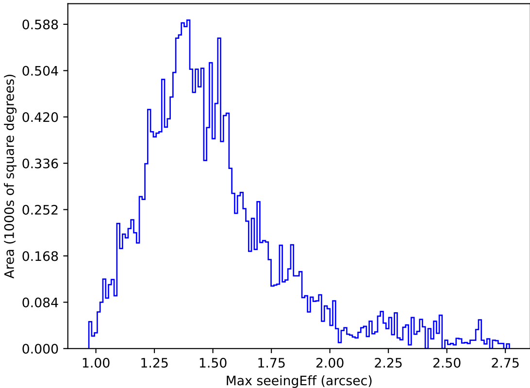
no_high_blob_v3.3_10yrs Yr 1 y band: Max seeingEff
