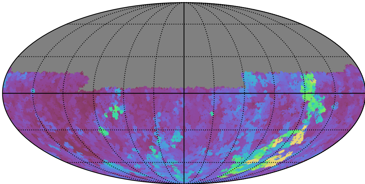
no_high_blob_v3.3_10yrs Yr 1 u band: Max seeingEff
