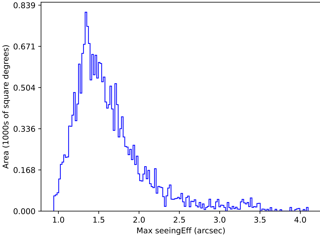
no_high_blob_v3.3_10yrs Yr 1 u band: Max seeingEff
