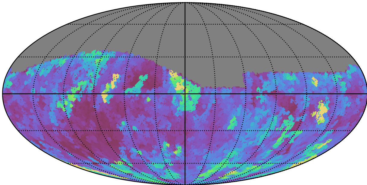
no_high_blob_v3.3_10yrs Yr 1 r band: Max seeingEff
