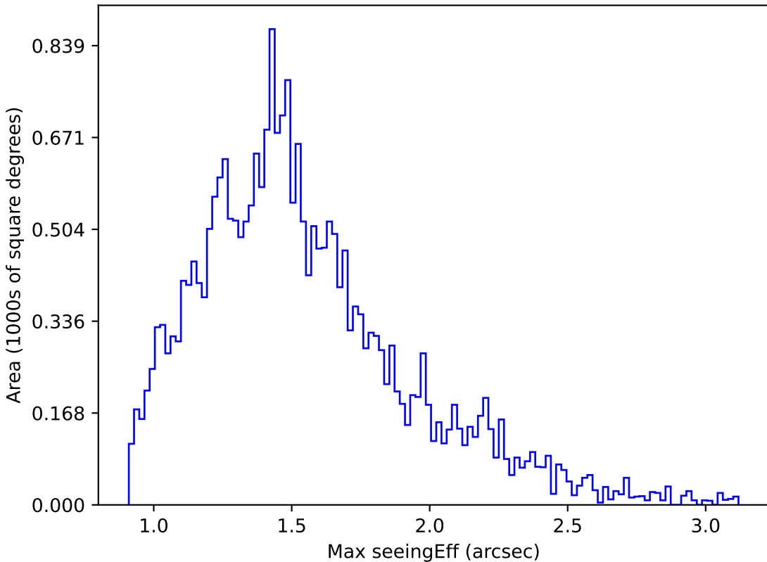
no_high_blob_v3.3_10yrs Yr 1 r band: Max seeingEff
