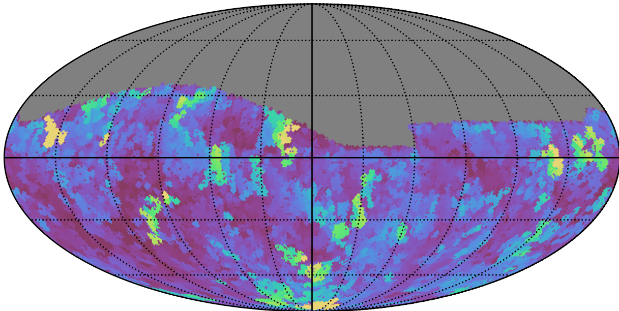
no_high_blob_v3.3_10yrs Yr 1 i band: Max seeingEff
