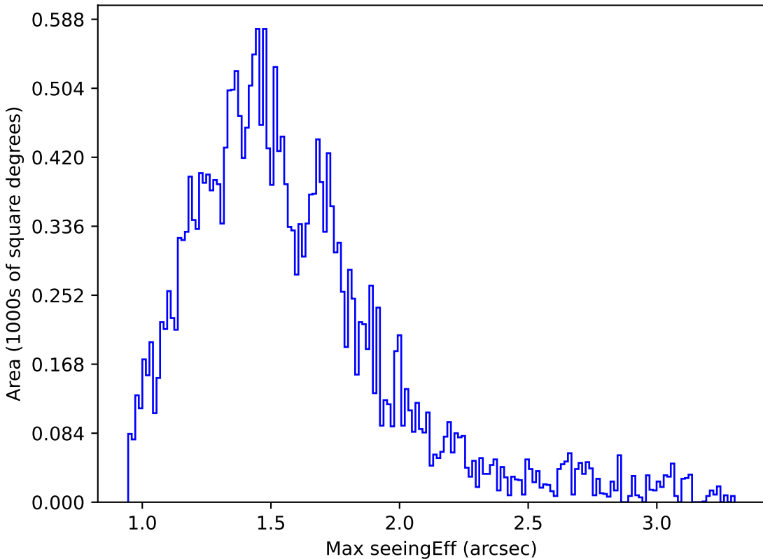
no_high_blob_v3.3_10yrs Yr 1 i band: Max seeingEff
